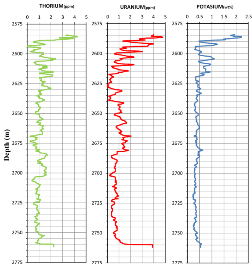
Fig. 9: Record of the Spectral Gamma Ray (SGR) log data (Thorium, Uranium, and Potassium curves) for the Kura China Formation A Unit in the well SH-4.
