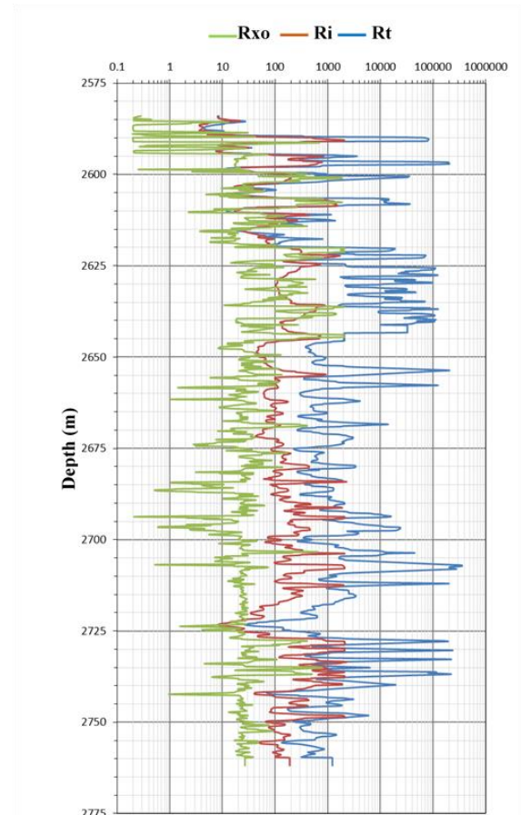
Fig. 14: Resistivity log record of Kurra Chine A Unit in SH-4.
