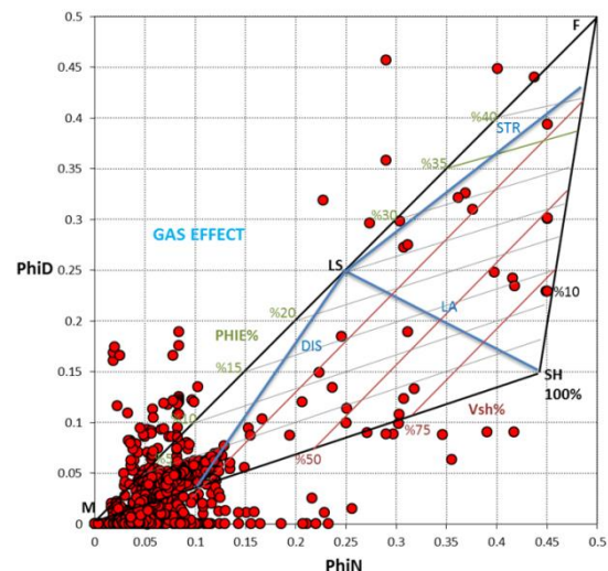
Fig. 13: Thomas-Stieber crossplot for determining mode of shale distribution for Kurra Chine A Unit in SH-4.
