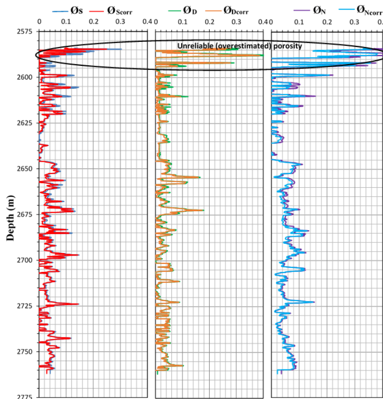
Fig. 11: Incorrected and corrected Sonic, Density, and Neutron porosities for Kurra China A Unit in SH-4.
