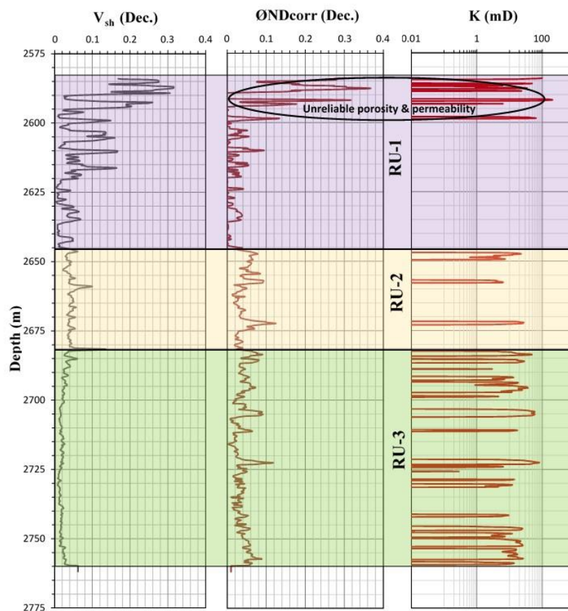
Fig. 19: Distinguished reservoir units for Kurra Chine A Unit in the well SH-4.
