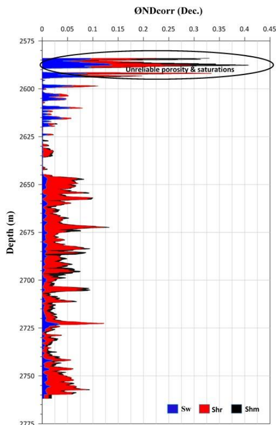
Fig. 16: Distribution of water, residual hydrocarbon, and movable hydrocarbon saturations within the pore spaces of Kurra Chine A Unit in SH-4 well.
