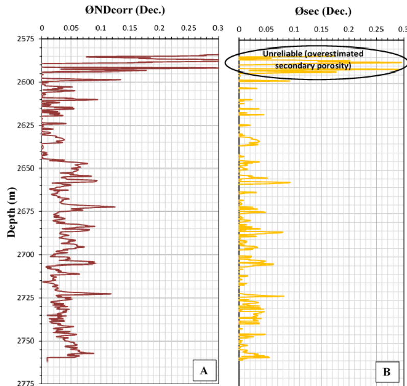
Fig. 12: A, Corrected Neutron-Density combination porosity ( \emptyset\text{NDcorr} ); B, Secondary porosity ( \emptyset\text{sec} ) for Kurra Chine A Unit in SH-4.
