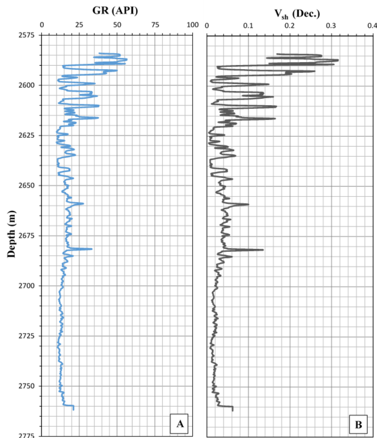
Fig. 8: A; Gamma ray record and B; calculated shale volume for Kurra Chine A Unit in SH-4.
