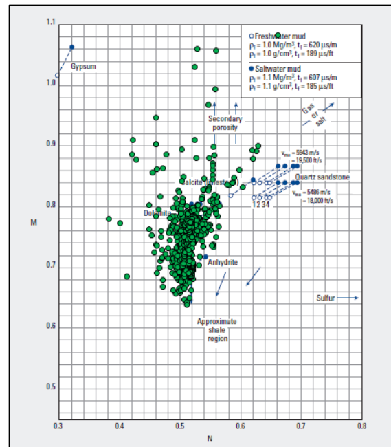
Fig. 6: M-N cross plot for determining lithology of the Kurra Chine A Unit in the well SH-4.
