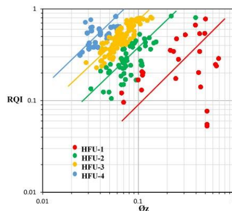
Fig. 21: Plot of RQI versus \phi_z for the studied Unit A of Kurra Chine Formation in the well SH-4 with the identified Hydraulic Flow Units (HFU).
