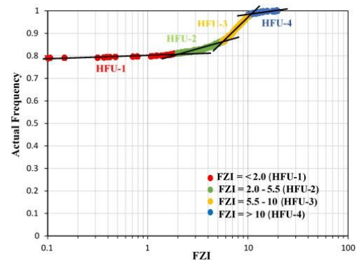
Fig. 20: Actual Frequency (distribution) of the calculated Flow Zone Indicators (FZI) for the studied Unit A of Kurra Chine Formation in the well SH-4 with the identified Hydraulic Flow Units (HFU).
