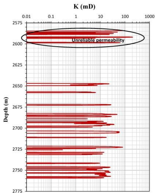
Fig. 18: Calculated Permeability (K) for the studied Kurra Chine A Unit in the well SH-4.
