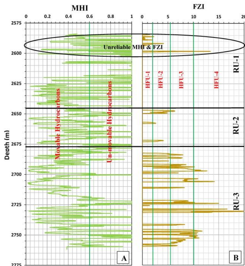
Fig. 22: A, Movable Hydrocarbon Index (MHI) and B, Flow Zone Indicator (FZI) for the distinguished reservoir units of Kurra Chine A Unit in the well SH-4.
