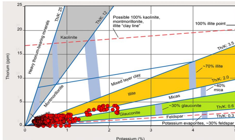
Fig. 10: Thorium - Potassium crossplot for identification of the clay minerals composing the shale content of the Kurra China A Unit in the well SH-4 (The crossplot is after [18]).
