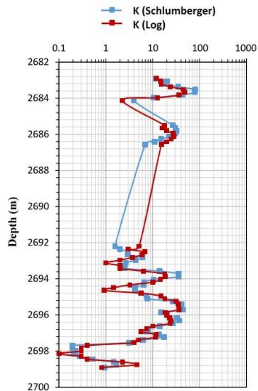
Fig. 17: Permeability estimation using Schlumberger equation and log data for a selected interval of Kurra Chine A Unit in the well SH-4.
