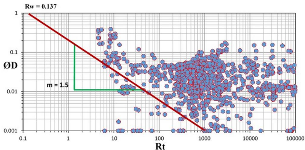
Fig. 15: Picket plot for determining cementation exponent ( m ) for Kurra Chine A Unit in SH-4.
