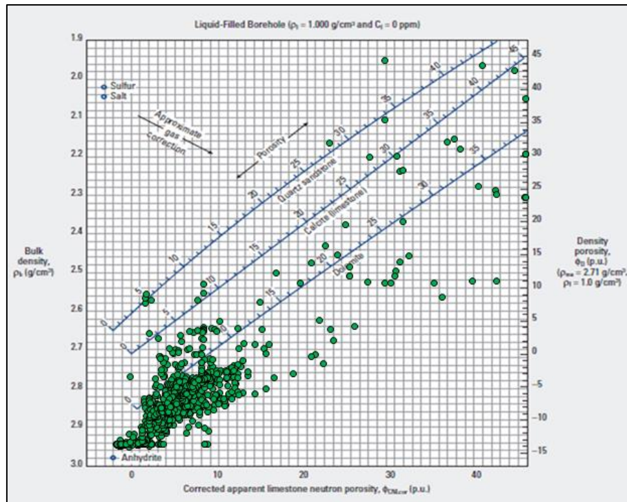
Fig. 5: Neutron-Density cross plot for determining lithology of the Kurra Chine A Unit in the well SH-4.
