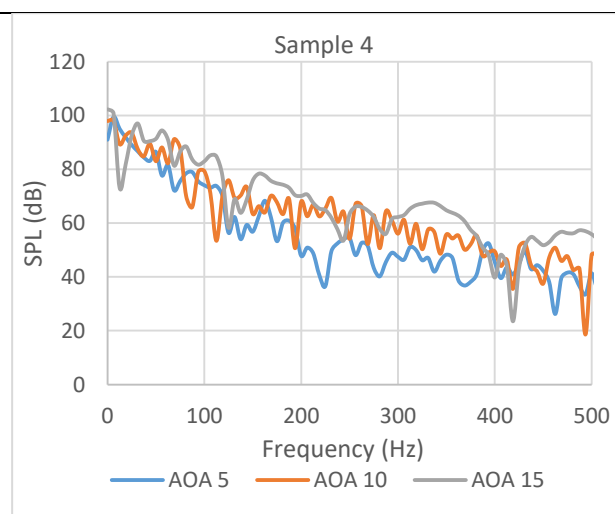
Figure 13. SPL vs. Freq. for sample4 for AOA 5,10, 15
