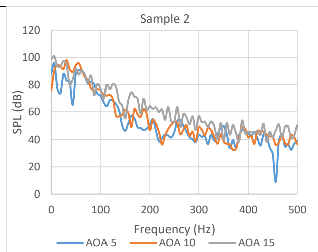
Figure 11. SPL vs. Freq. for sample2 for AOA 5,10, 15
