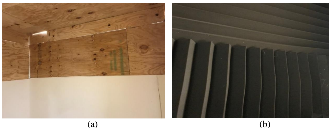
Figure 1. a) The first layer of foam (Volara Foam), b) The second layer of foam (Wedge Foam)
