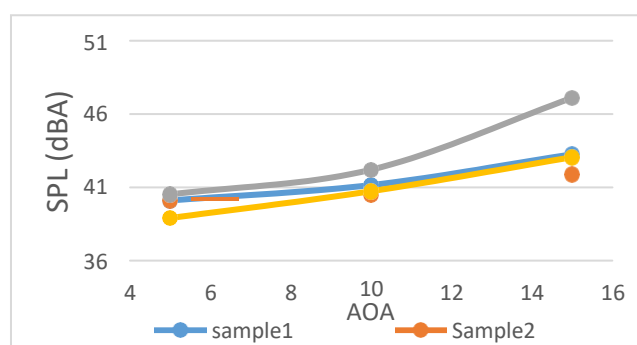
Figure 14. The overall sound level for all samples vs. AOA
