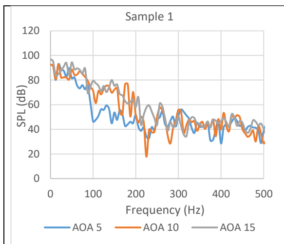
Figure 10. SPL vs. Freq. for sample1 for AOA 5,10, 15
