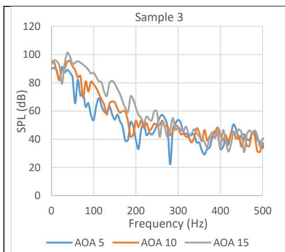
Figure 12. SPL vs. Freq. for sample3 for AOA 5,10, 15
